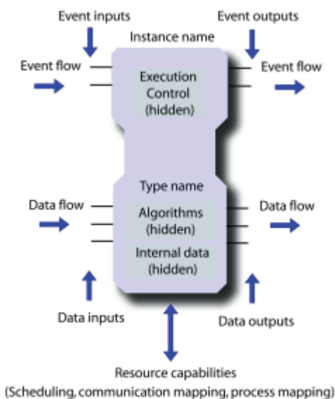
Figure 1: IEC 61499 Function Block Model
