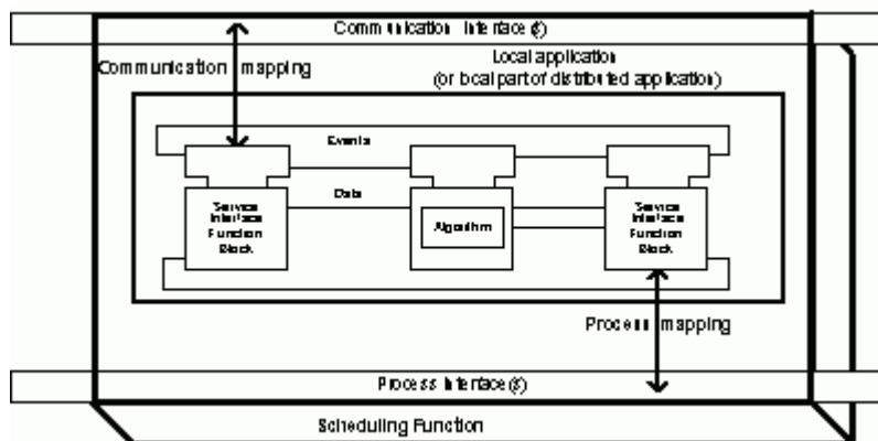
Figure 1: IEC 61499 Resource Model
