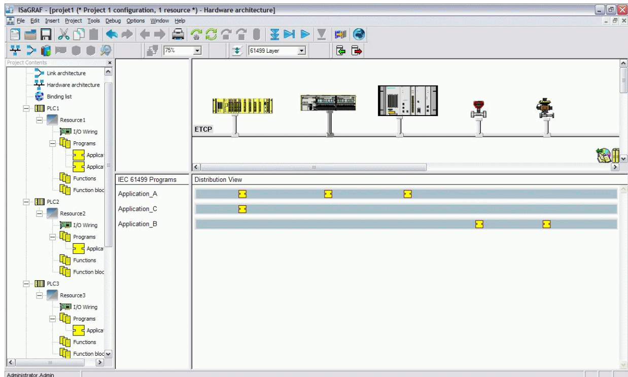
Figure 2: ISaGRAF system model viewer
