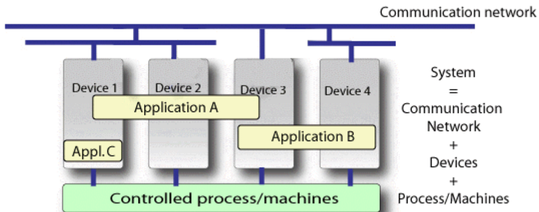
Figure 1: The IEC 61499 system model
